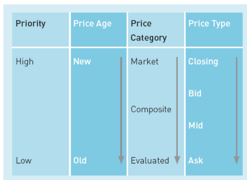
Figure 8-2. Price weighting
