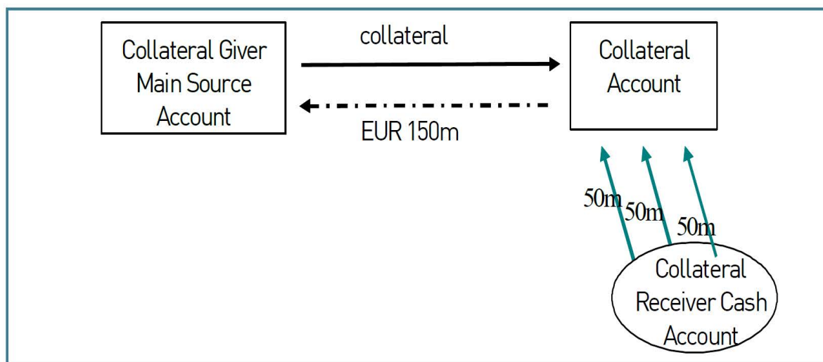
Figure 4-4. Cash shaping
